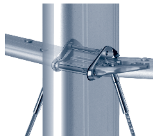
Through-bar spreader bracket, incorporates attachments for lower shrouds or intermediate shrouds.
