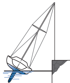
30° heeling test.
