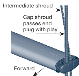
Intermediate shroud Cap shroud passes end plug with play Forward Spreader end plug for continuous rigging.
